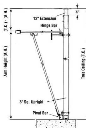
Standard Installation - True Ceiling Min. 14" above arm height
