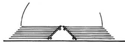
"V" Plans and Angle Plans - "V" and Angle Plans allow arms to fold flat along the wall for compact storage. Specify type 103-B racks.
