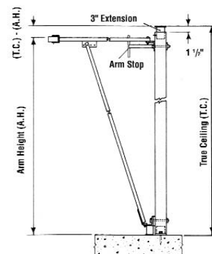
Low Ceiling Installation - True Ceiling Min. 3" above arm height
