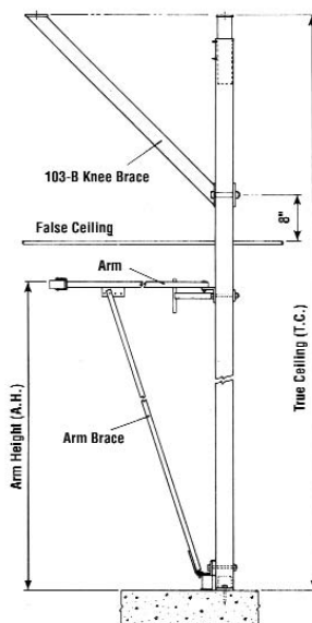
High Ceiling Installation - Uprights exceed 36" above arm height
